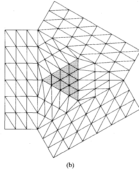
Fig. 2. Typical divisions for H -plane waveguide junctions with a ferrite post. (a) Circular ferrite post. (b) Triangular ferrite post.
