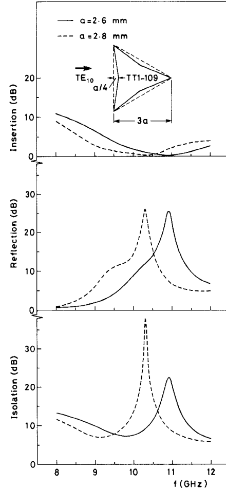
Fig. 8 Performance of a Y-junction with a TT1-109 triangular ferrite post having depressed sides for the second arrangement.
