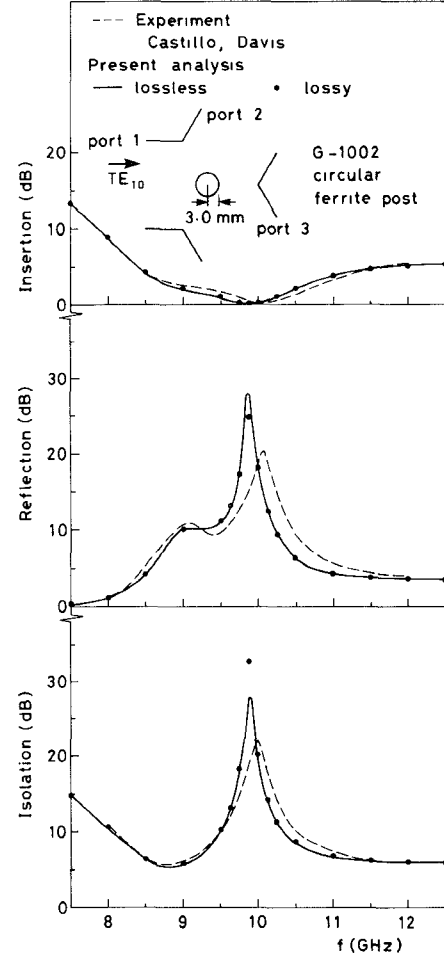
Fig. 4. Performance of a Y-junction with a G-1002 circular ferrite post.
